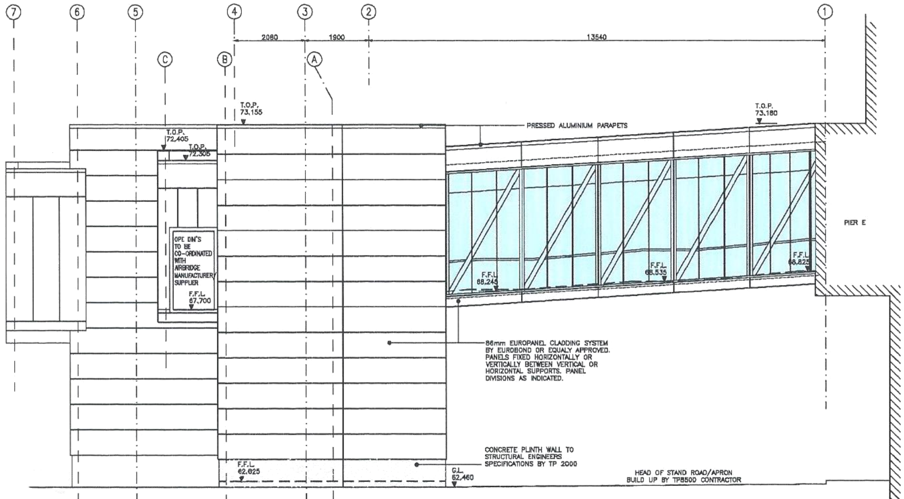
GATE 10 - ELEVATION 2
