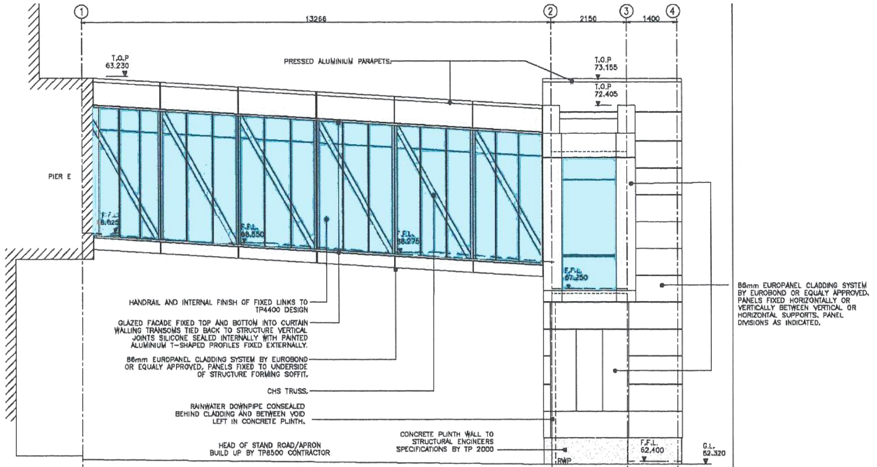
GATE 11 - ELEVATION 1
