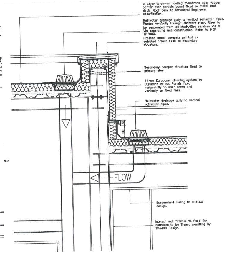
TYPICAL CORRIDOR ROOF DETAIL 2
