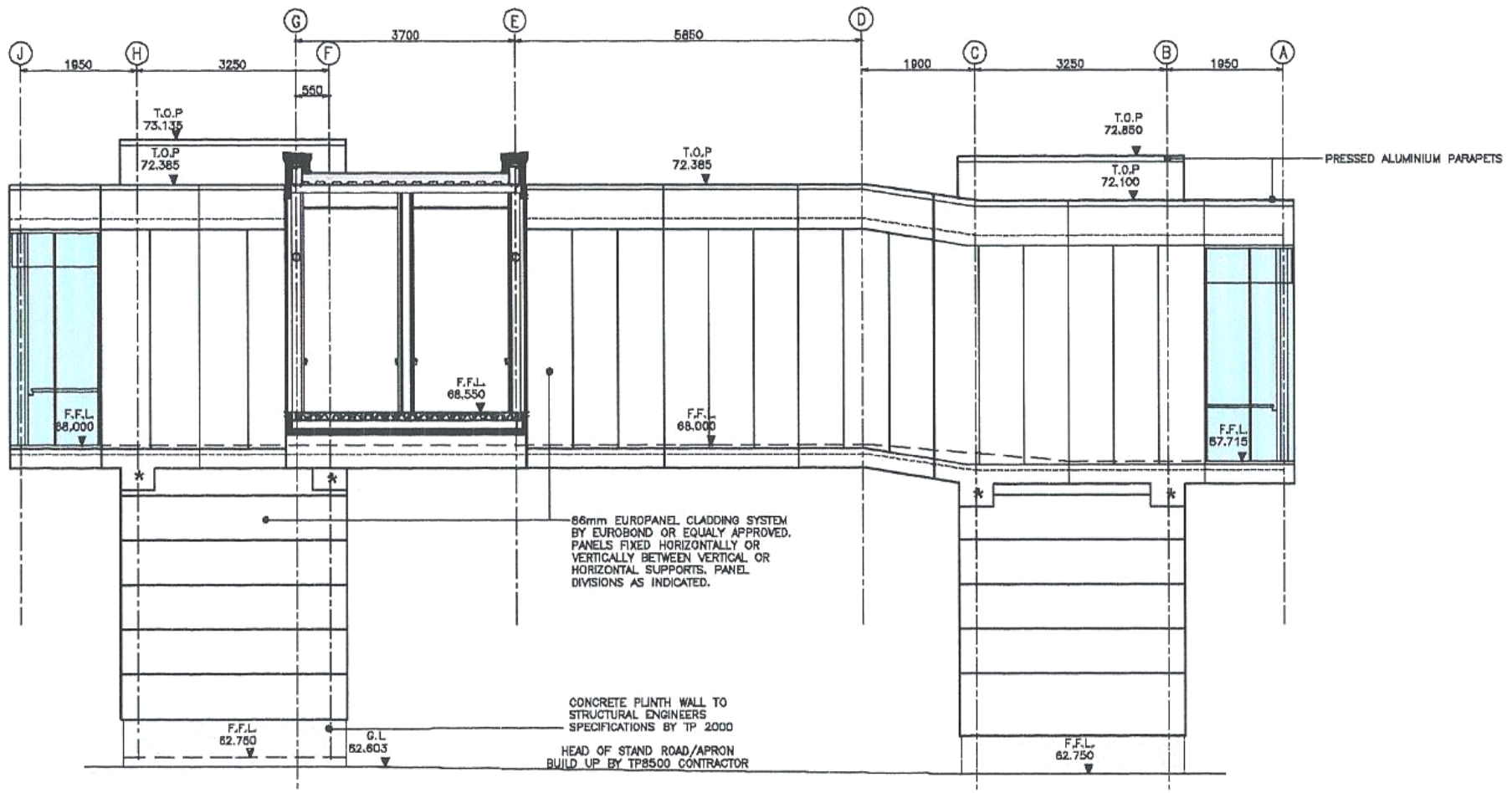
GATE 9 - ELEVATION 4
