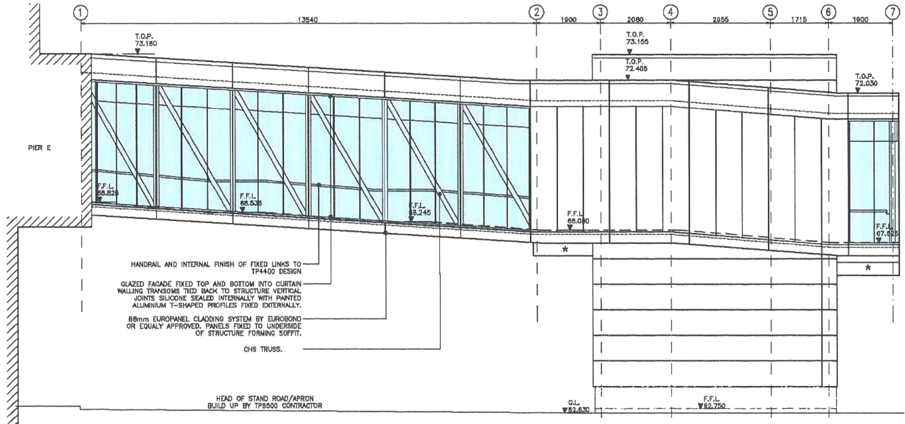
GATE 9 - ELEVATION 1
