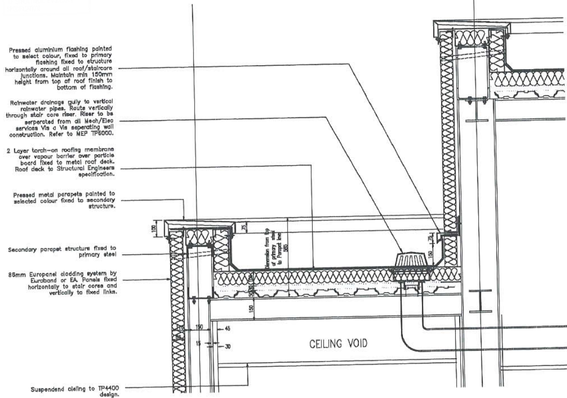
TYPICAL CORRIDOR ROOF DETAIL 1
