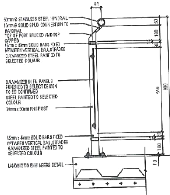
TYPICAL STAIR HANDRAIL SECTION OF BALUSTRADE
