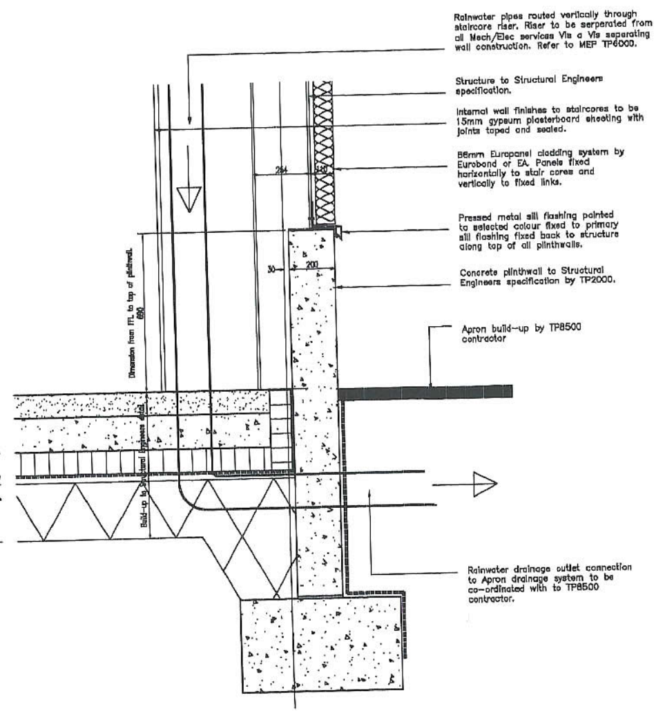
PLINTH WALL DETAIL 2
