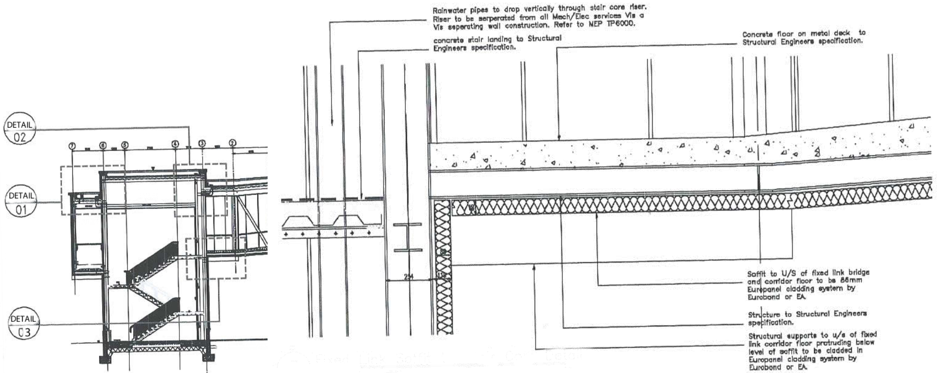
TYPICAL CORRIDOR ROOF DETAIL KEY
