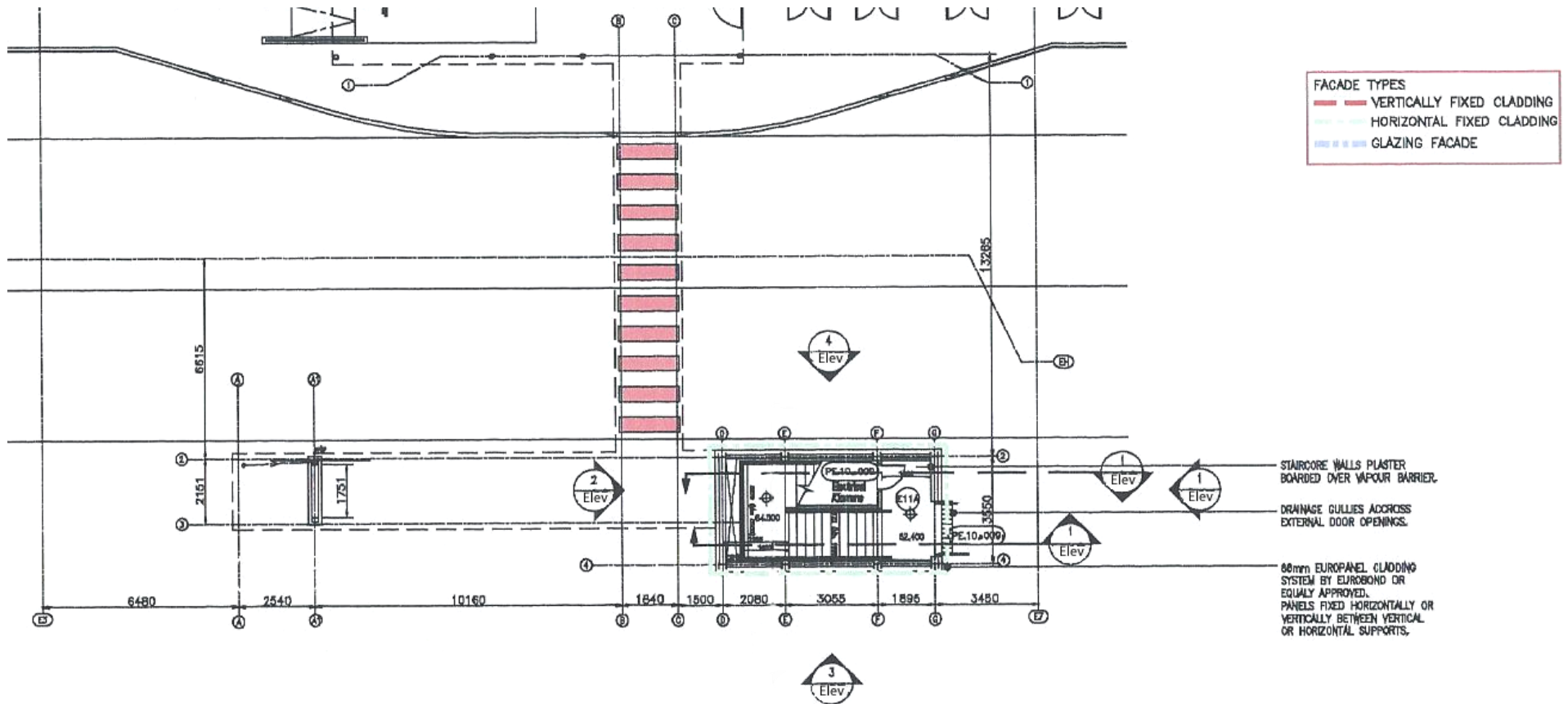
FIXED LINK TUNNEL & NODE BUILDING - GATE 11
