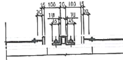
TYPICAL STAIR HANDRAIL DTAIL 5
