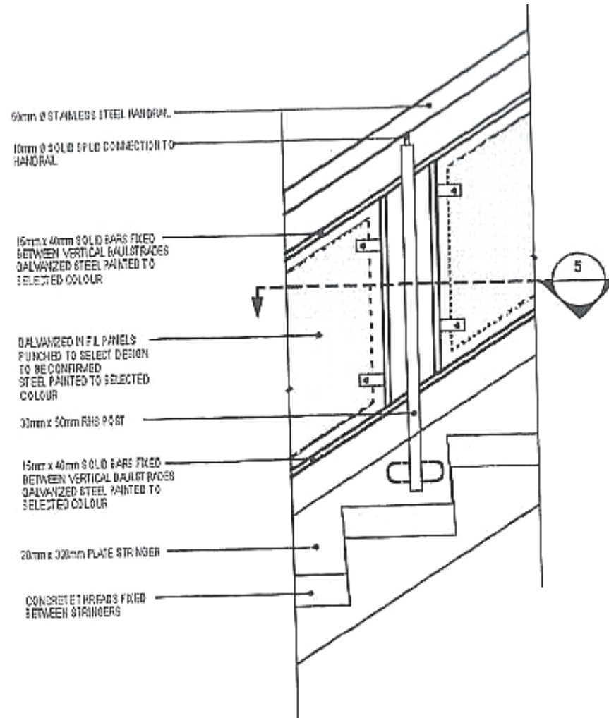
TYPICAL STAIR HANDRAIL SECTION SHOWING MID BALUSTRADE
