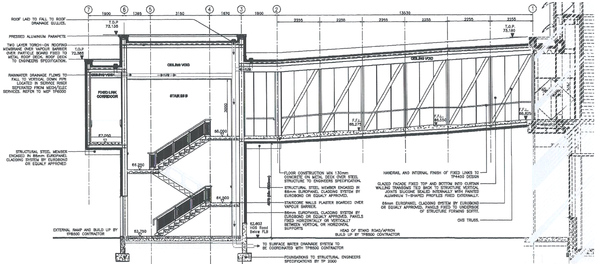
GATE 9 - SECTION
