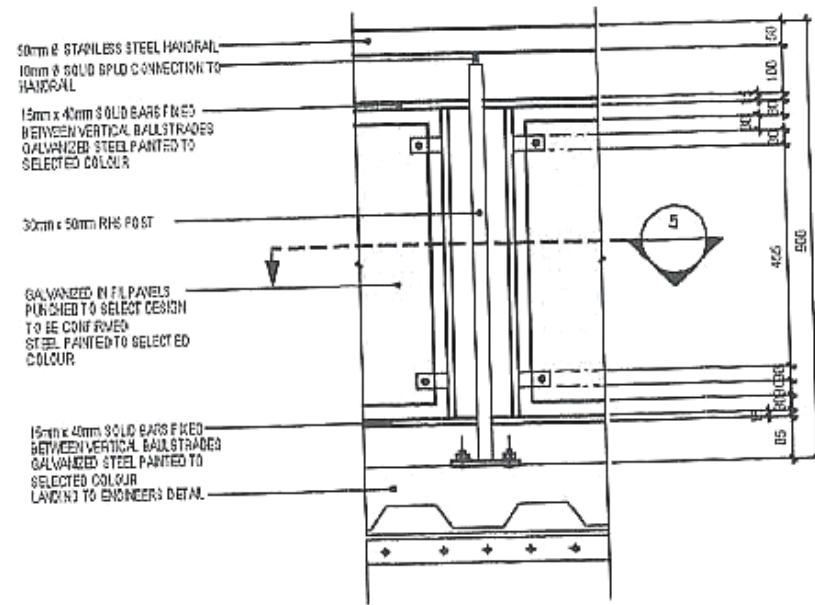
TYPICAL STAIR HANDRAIL ELEVATION OF BALUSTRADE
