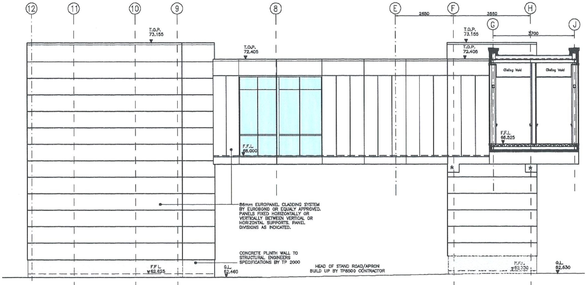
GATE 10 - ELEVATION 3
