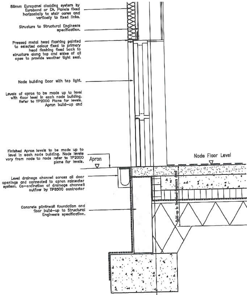
PLINTH WALL DETAIL 1
