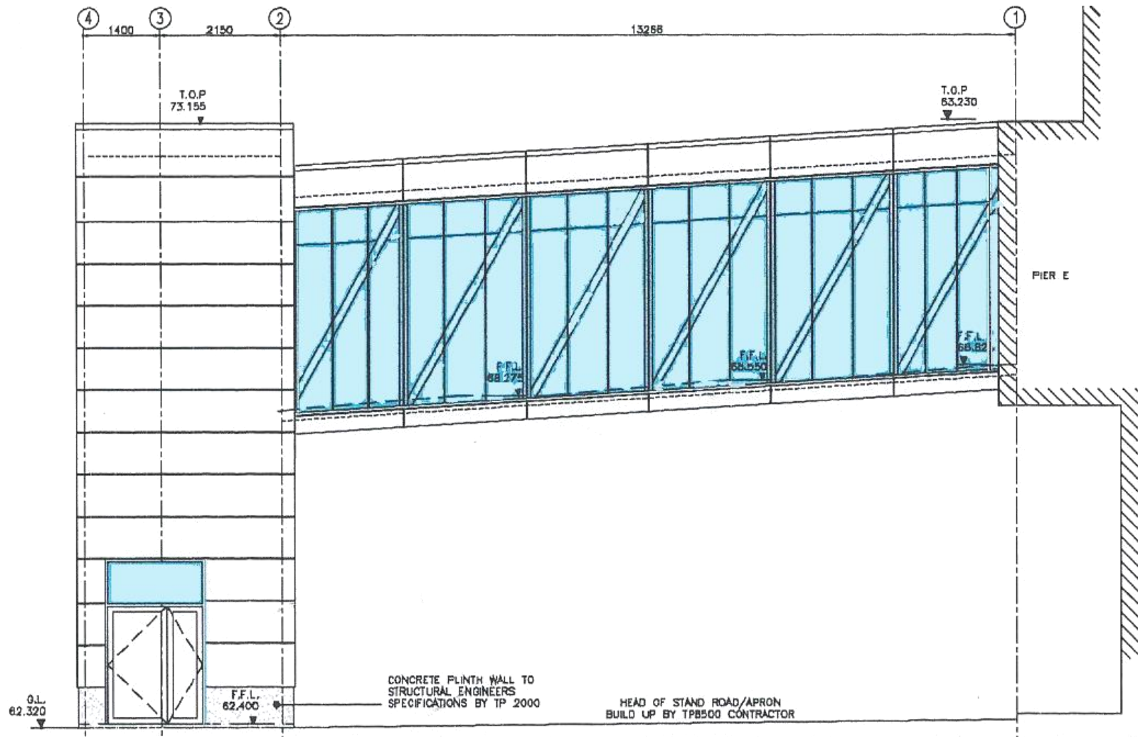
GATE 11 - ELEVATION 2
