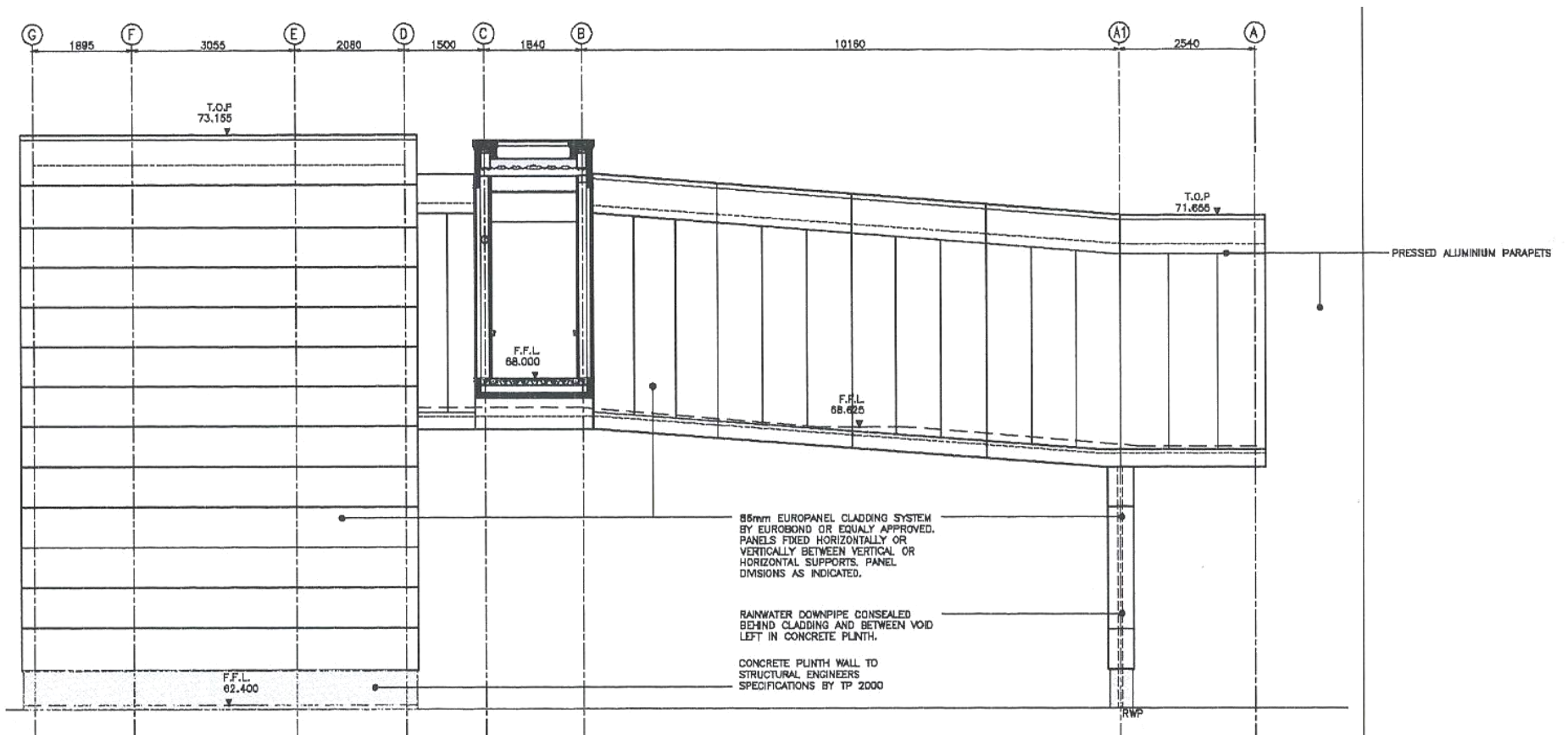
GATE 11 - ELEVATION 4
