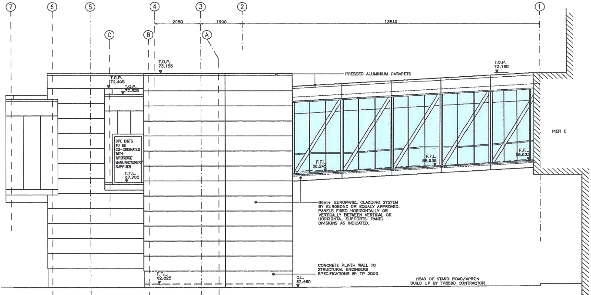
GATE 9 - ELEVATION 2
