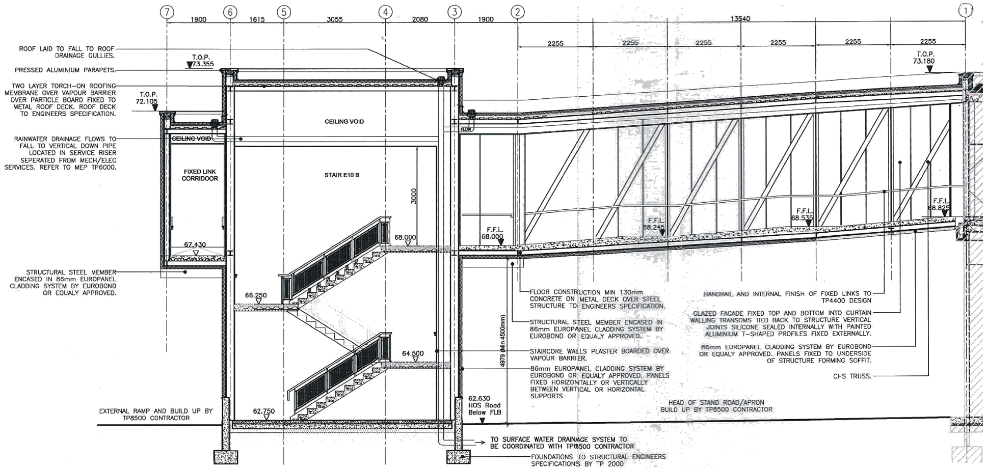
GATE 10 - SECTION
