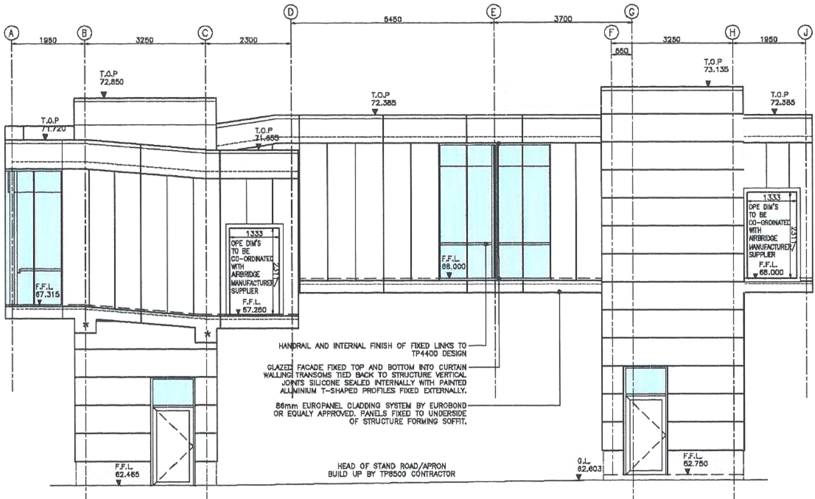
GATE 9 - ELEVATION 3
