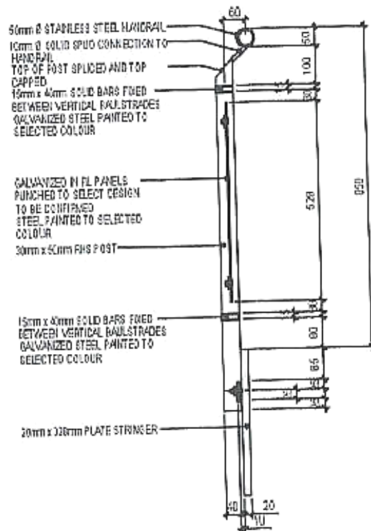
TYPICAL STAIR HANDRAIL SECTION THROUGH BALUSTRADE
