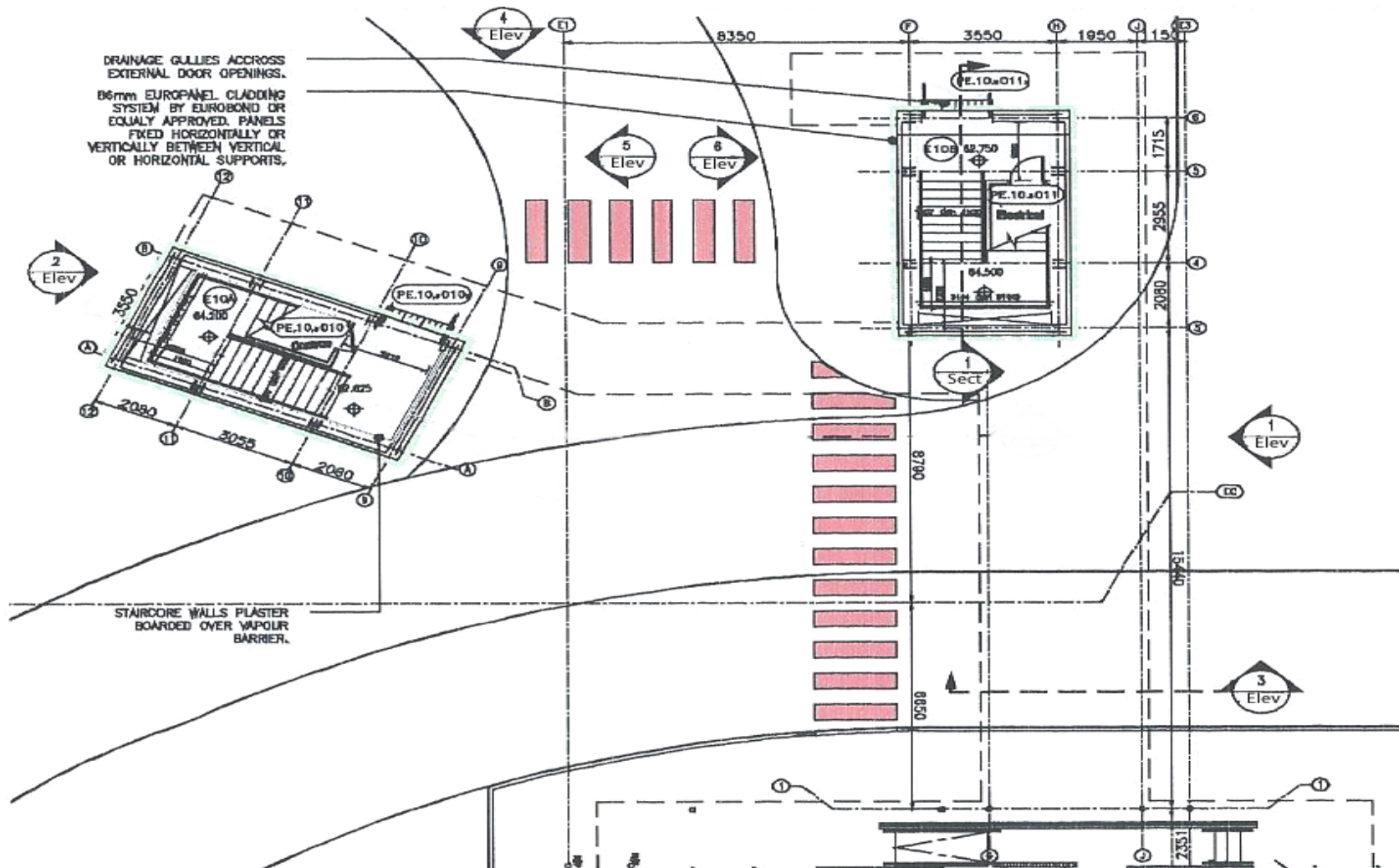
FIXED LINK TUNNEL & NODE BUILDING - GATE 10
