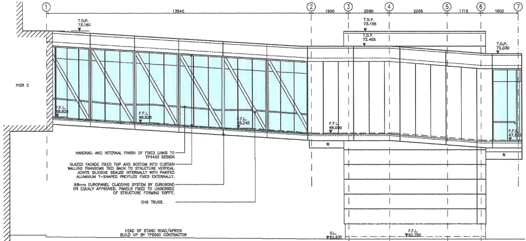
GATE 10 - ELEVATION 1
