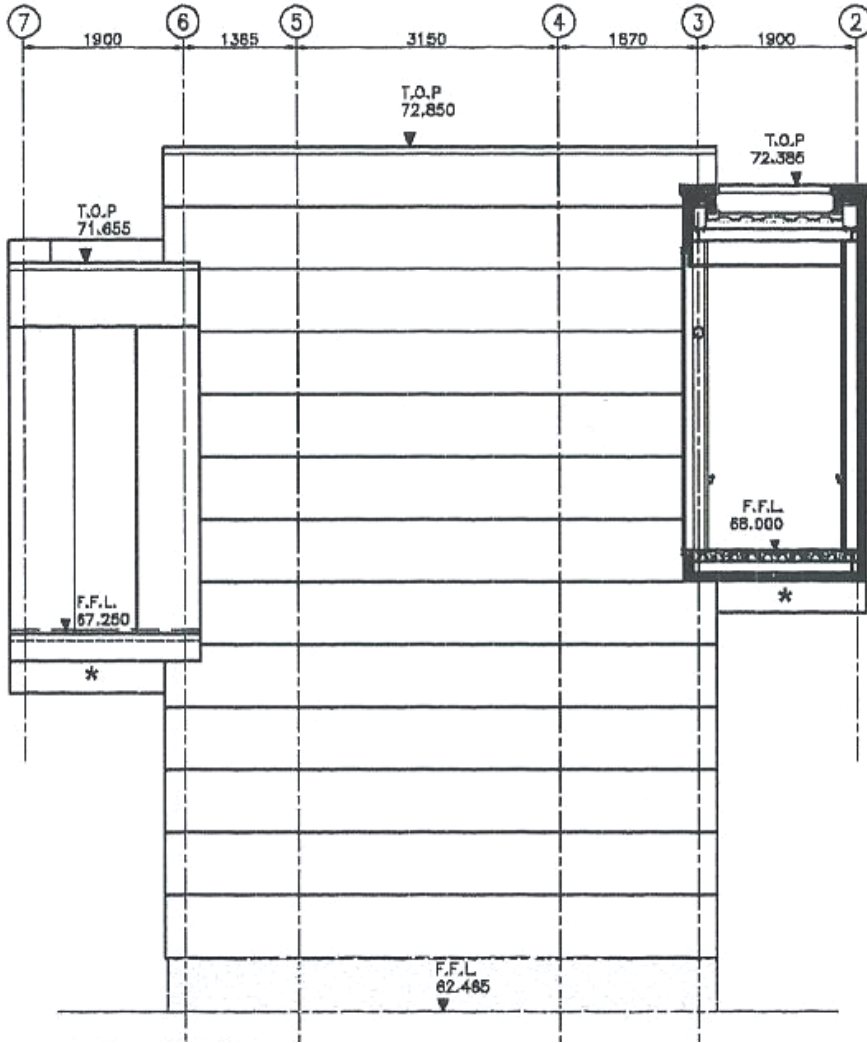
GATE 9 - ELEVATION 5
