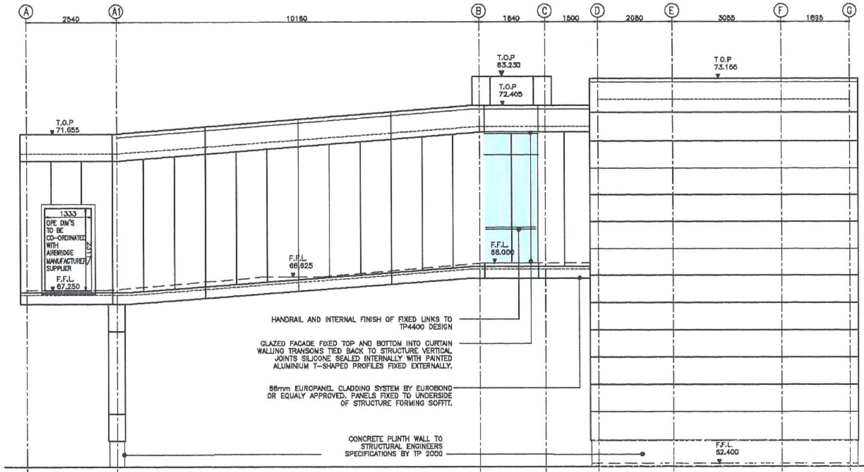
GATE 11 - ELEVATION 3
