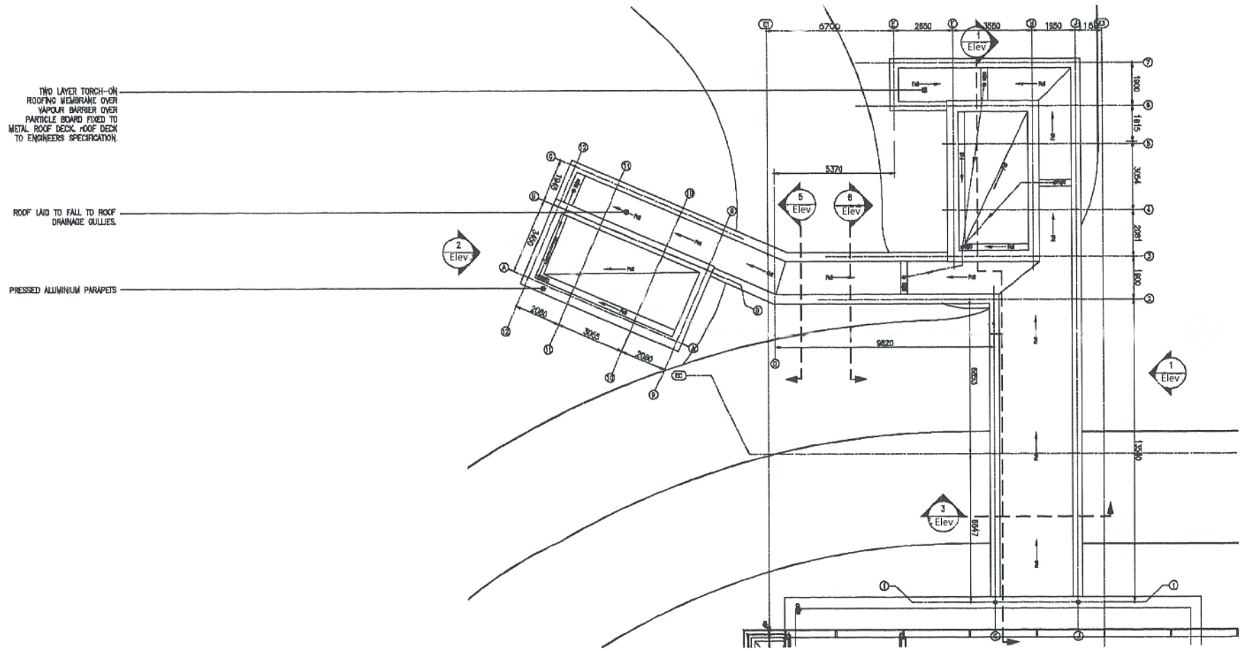
FIXED LINK TUNNEL & NODE BUILDING - GATE 10
