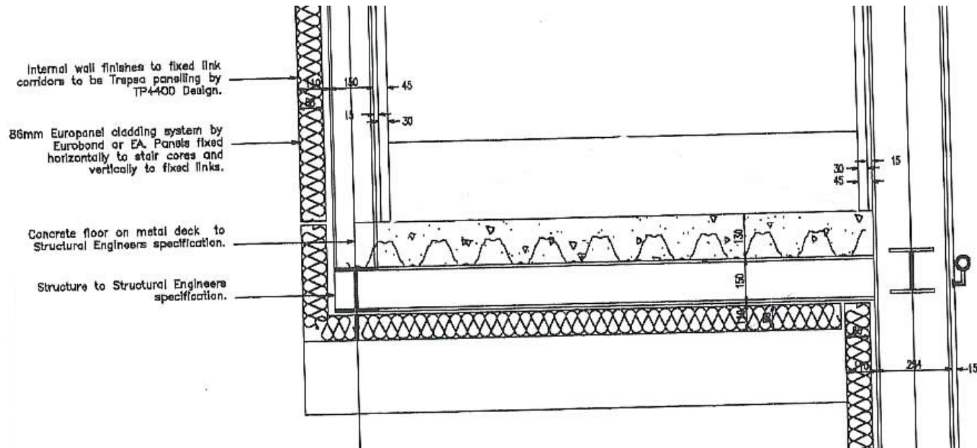
TYPICAL WALL BUILDUP DETAIL 3
