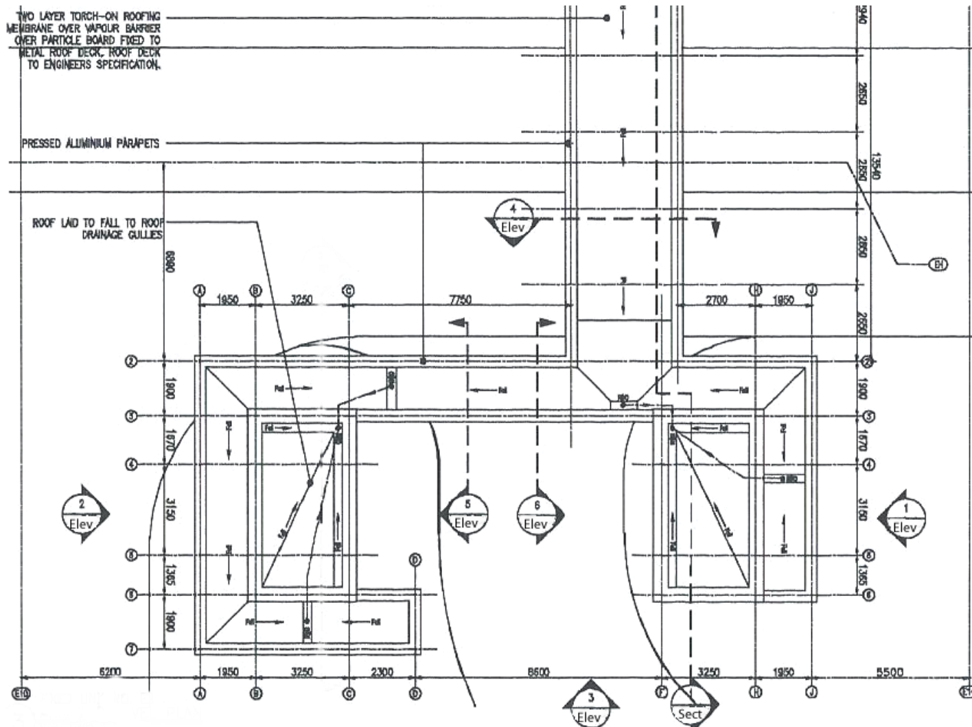
FIXED LINK TUNNEL & NODE BUILDING - GATE 9
