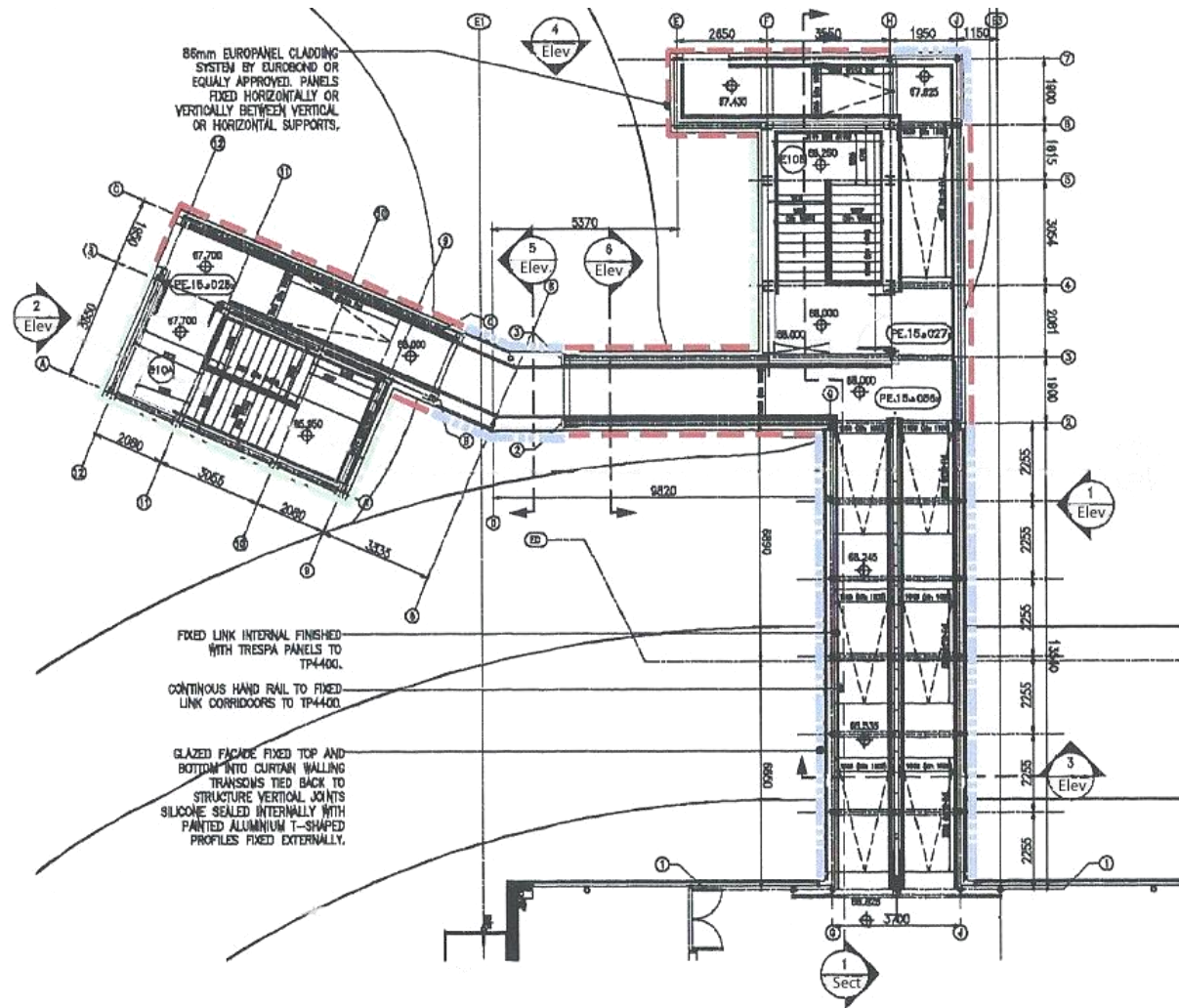
FIXED LINK TUNNEL & NODE BUILDING - GATE 10
