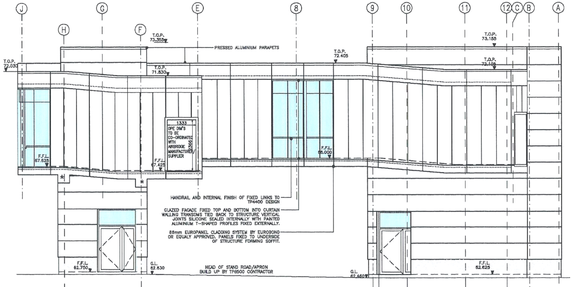
GATE 10 - ELEVATION 4
