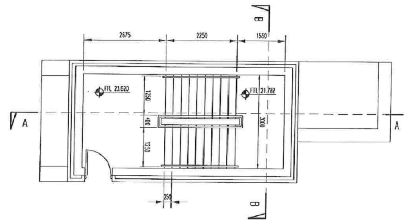
FIFTH FLOOR STAIR CORE
