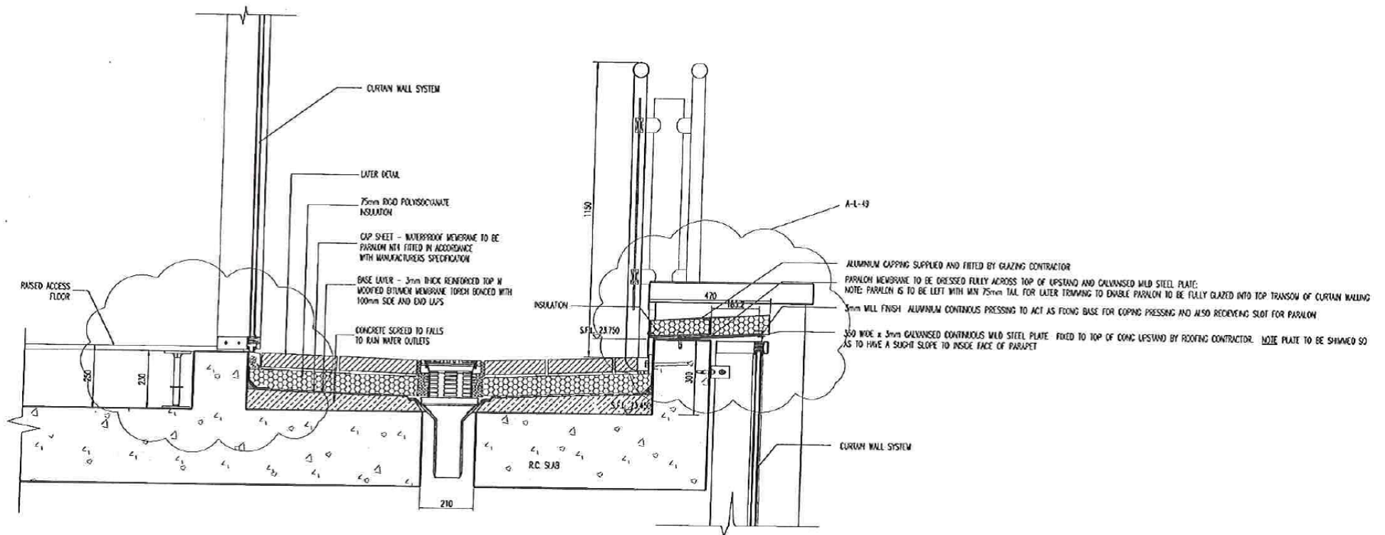
SECTION 18-18 BALCONY BUILD-UP AND RAIN WATER DRAINAGE
