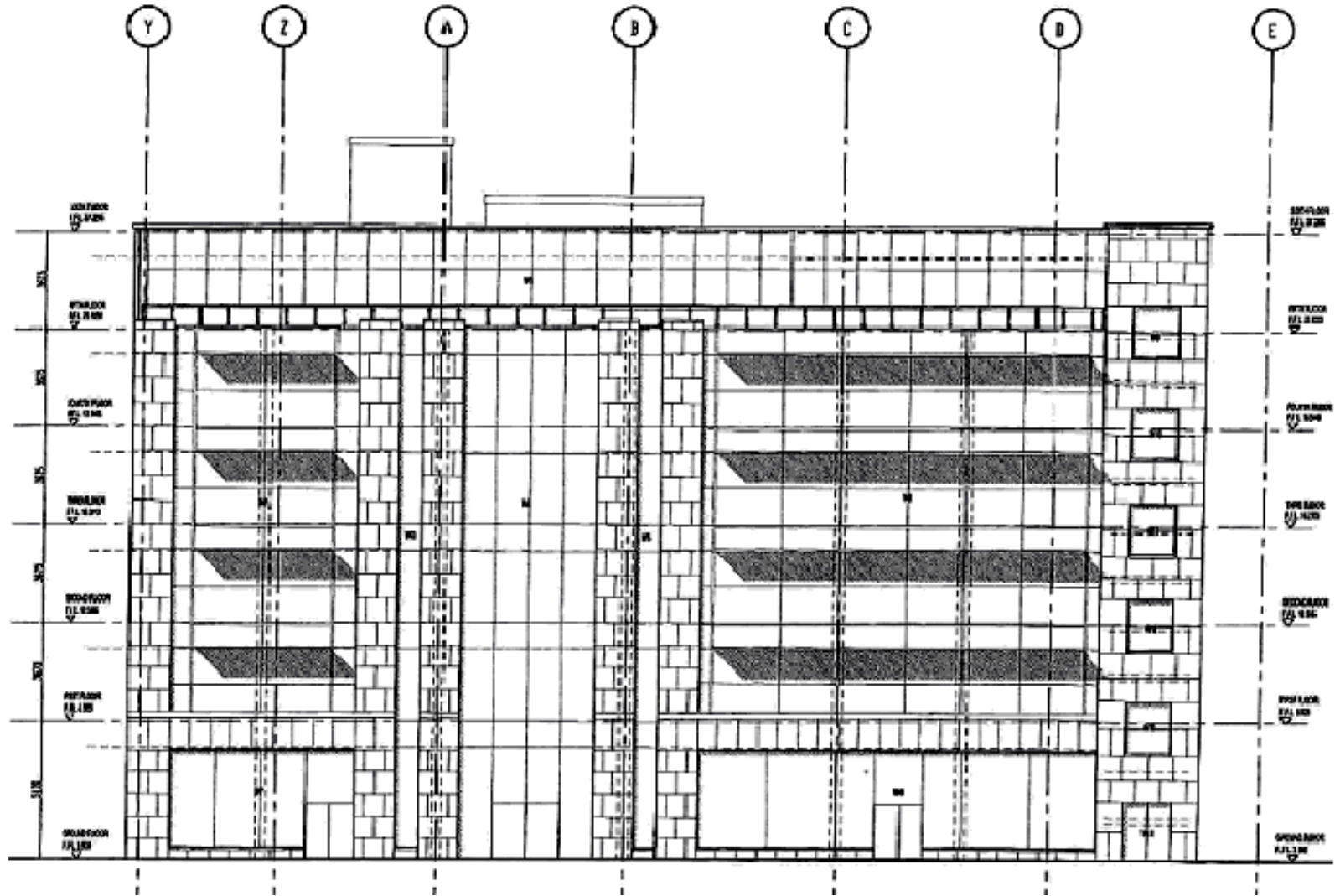
SOUTH ELEVATION
