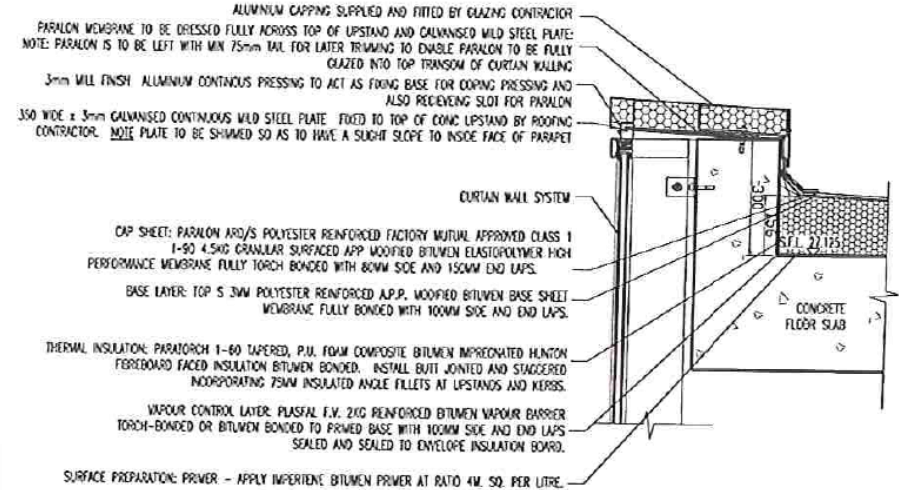
SECTION 12-12 TYPICAL PARAPET DETAIL CURTAIN WALL GLAZING
