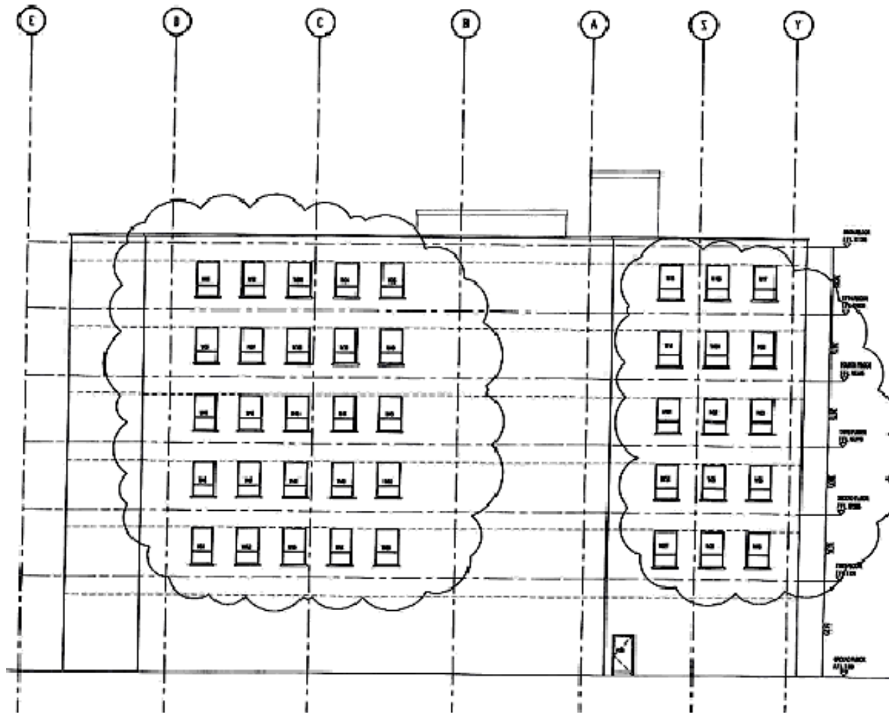
NORTH ELEVATION
