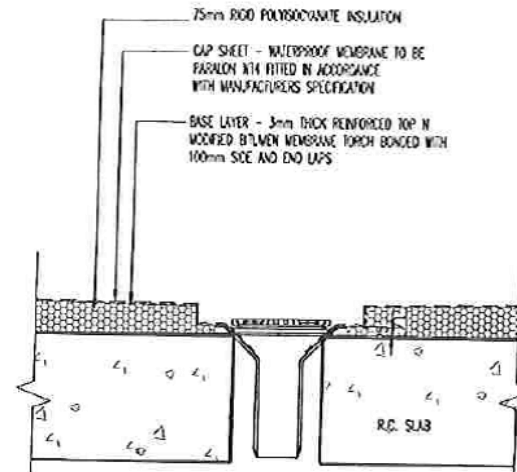
SECTION 21-21 TYPICAL ROOF INSULATION BUILD-UP AND RAIN WATER DRAINAGE
