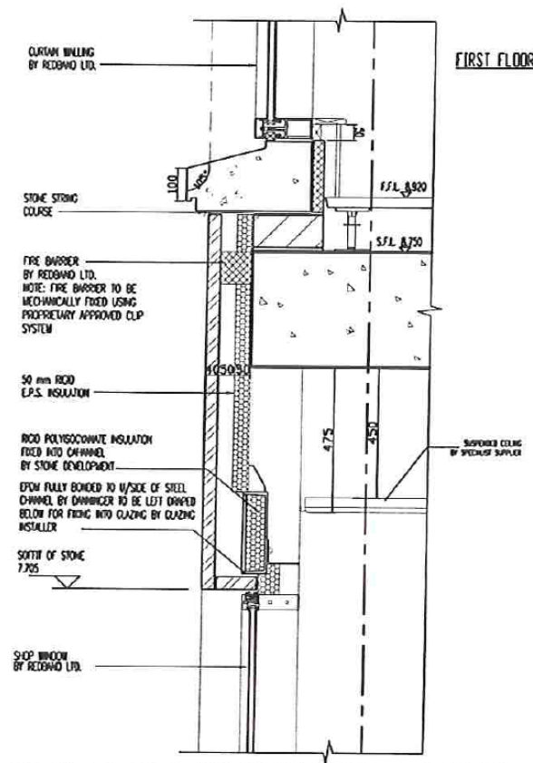
SECTION 8-8 TYPICAL SECTION THROUGH HEAD
