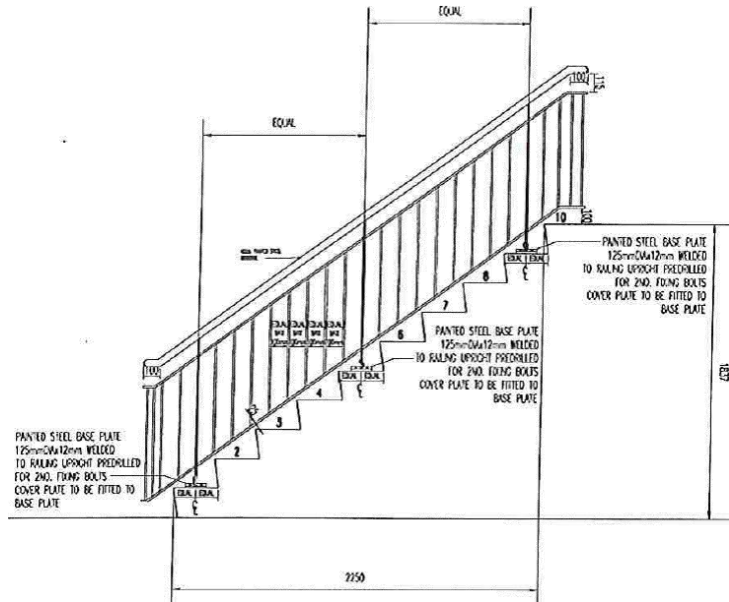
TYPICAL HAND RAIL DETAIL
