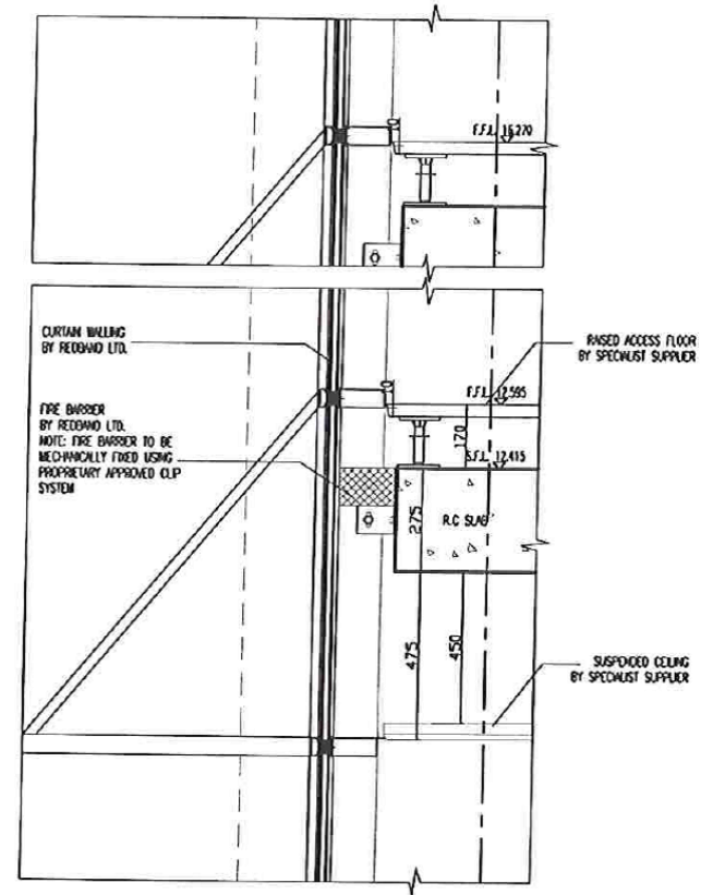
SECTION 9-9 TYPICAL SECTION THROUGH CURTAIN WALLING
