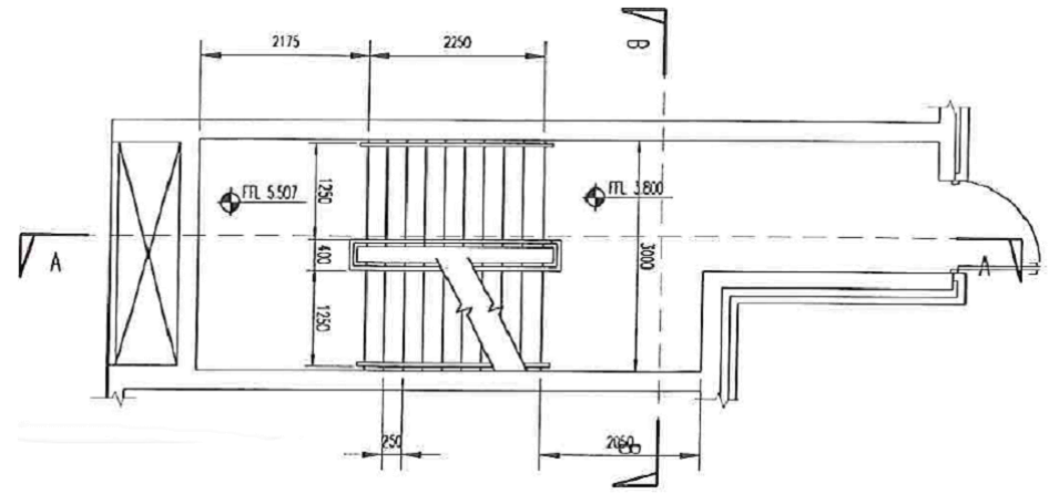
GROUND FLOOR STAIR CORE
