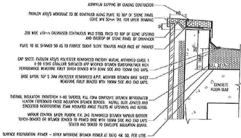
SECTION 19-19 TYPICAL PARAPET DETAIL CONCRETE STAIR CORE AND STONE
