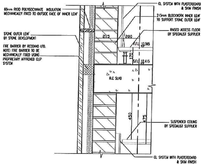
SECTION 11-11 TYPICAL SECTION THROUGH STONE
