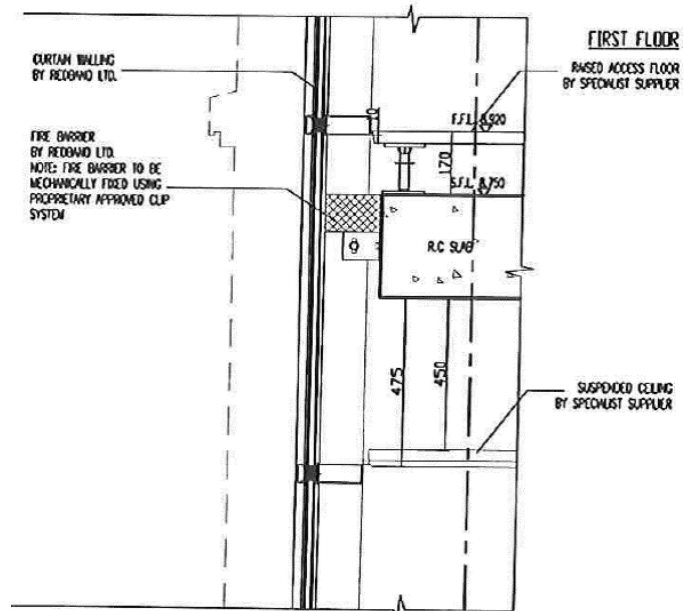
SECTION 12-12 TYPICAL SECTION THROUGH CURTAIN WALLING
