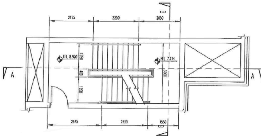
FIRST TO FOURTH FLOOR STAIR CORE
