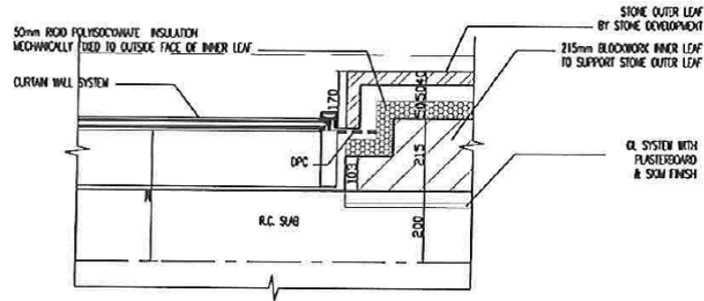
SECTION 10-10 TYPICAL SECTION THROUGH STONE, BLOCK AND CURTAIN WALLING
