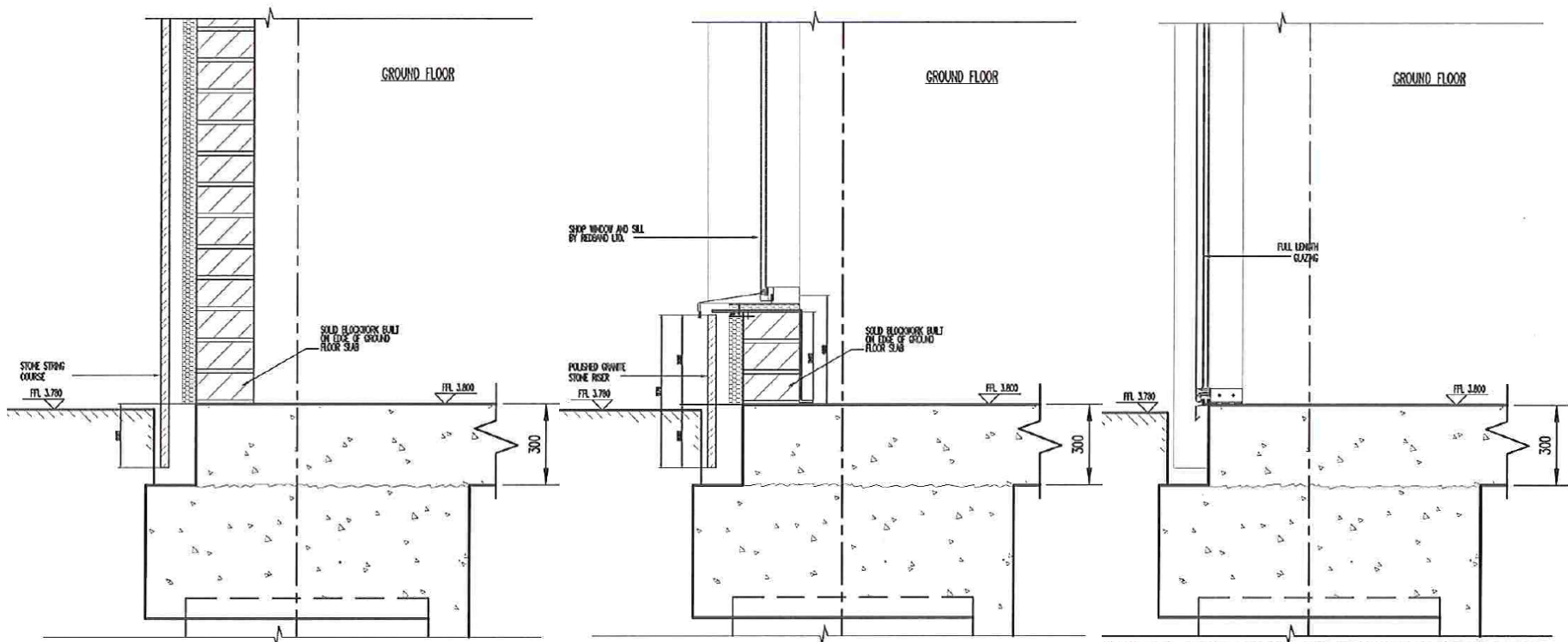
SECTION 1-1 TYPICAL SECTION THROUGH SHOP FRONT
