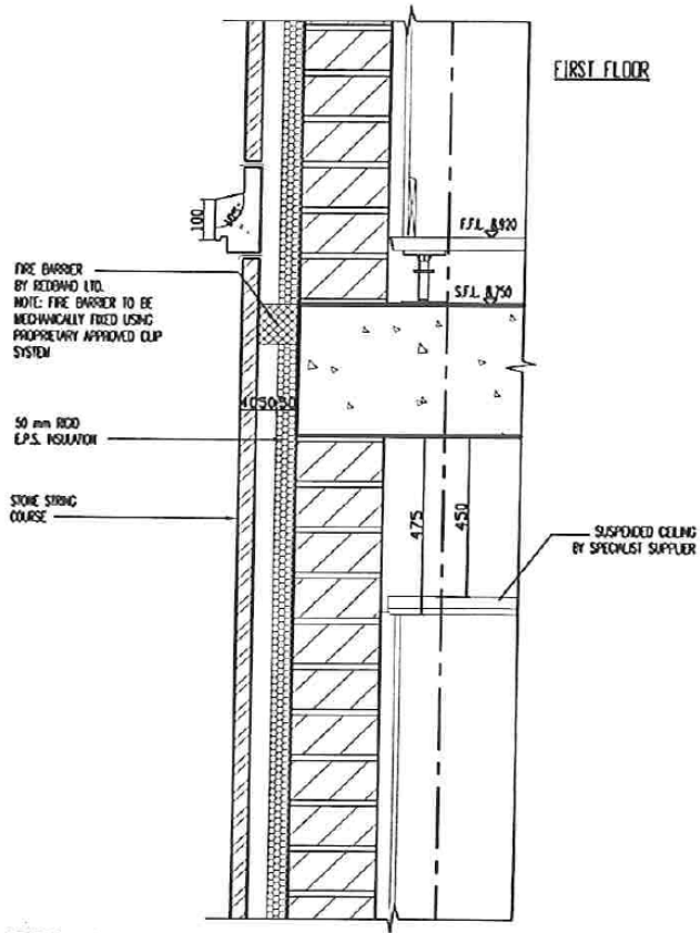
SECTION 7-7 TYPICAL SECTION THROUGH HEAD
