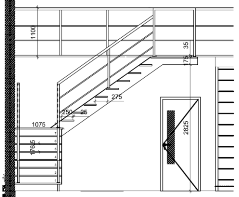
Steel Stair Type 2 - Section A-A
