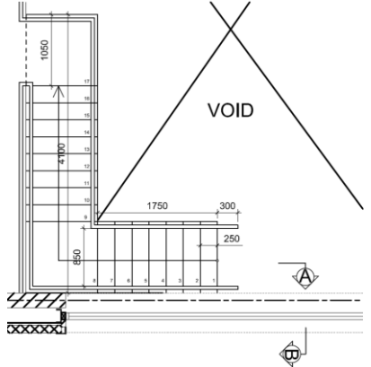
Steel Stair Type 2 - Plan - First Floor
