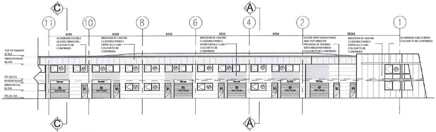
Elevation E-E
