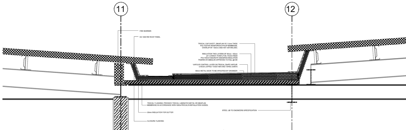
Gutter Detail
