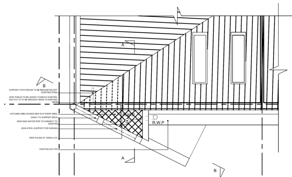
Flat Roof Detail - Typical Part Plan
