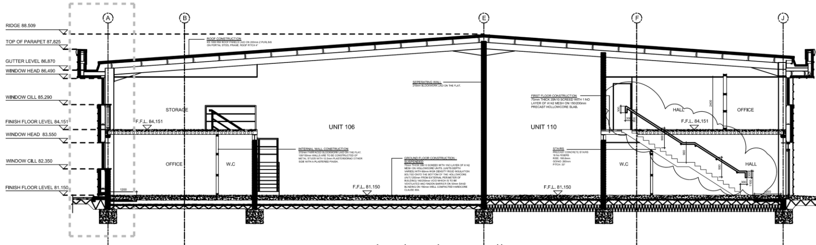
Section A-A - Dashed line shows Wall Section 1
