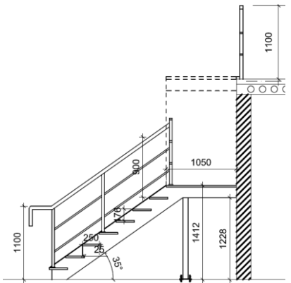
Steel Stair Type 2 - Section B-B
