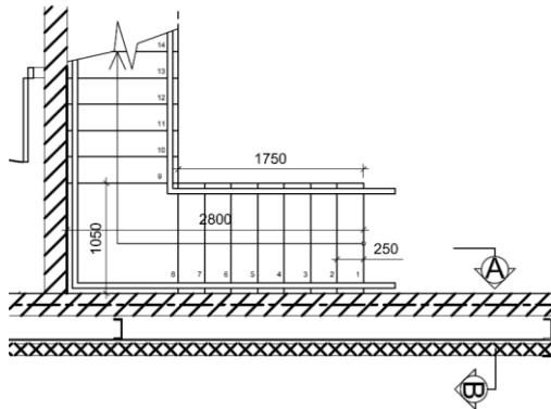
Steel Stair Type 2 - Plan - Ground Floor
