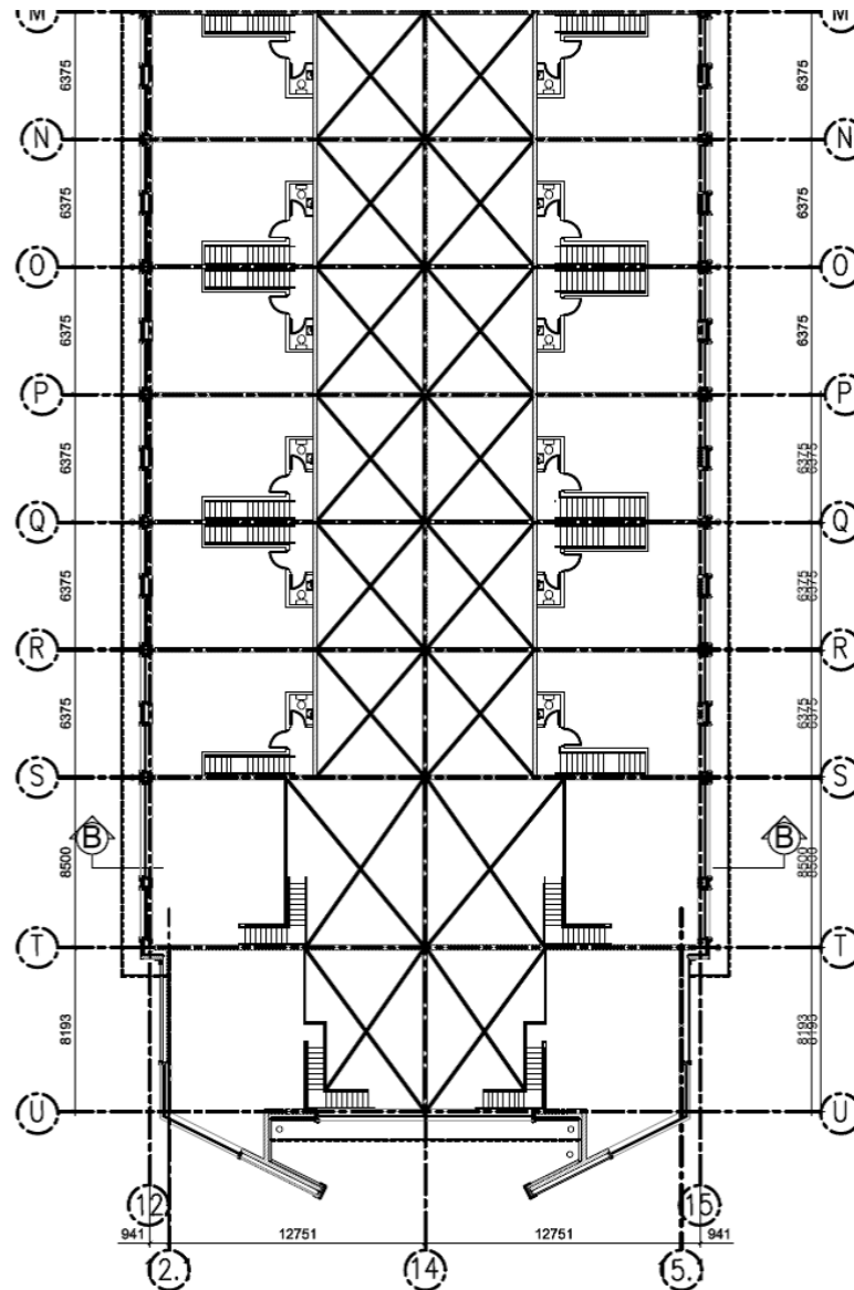
First Floor Plan 2 - Cut Through Grid Line M-M
