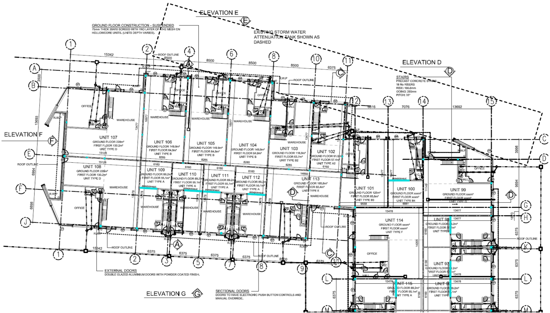
Ground Floor Plan 1 - Cut Through Grid Line M-M
