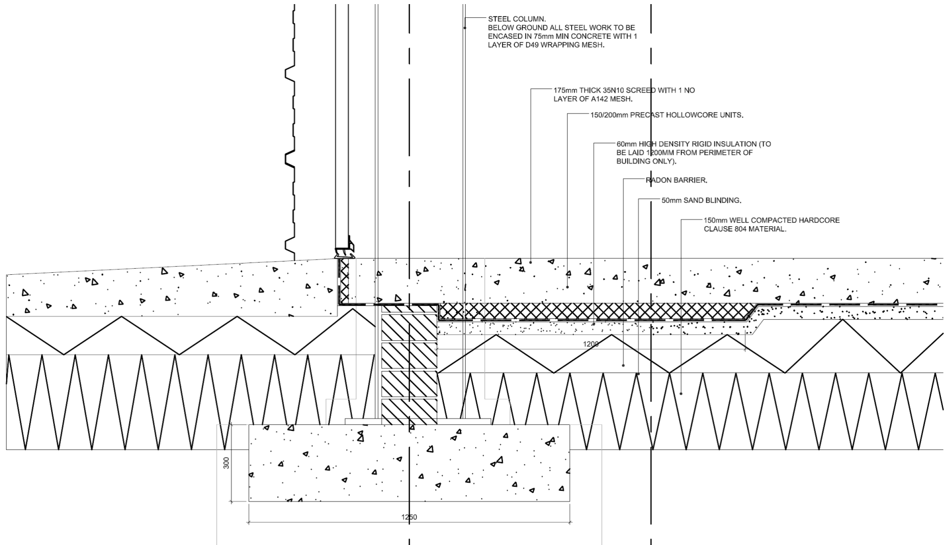
Detail 2
