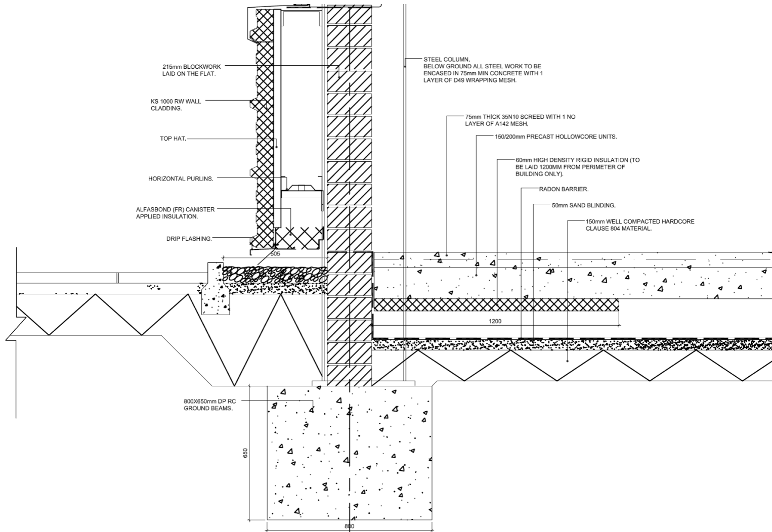
Detail 1
