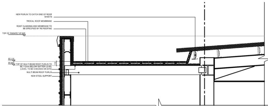
Flat Roof Detail - Section A-A
