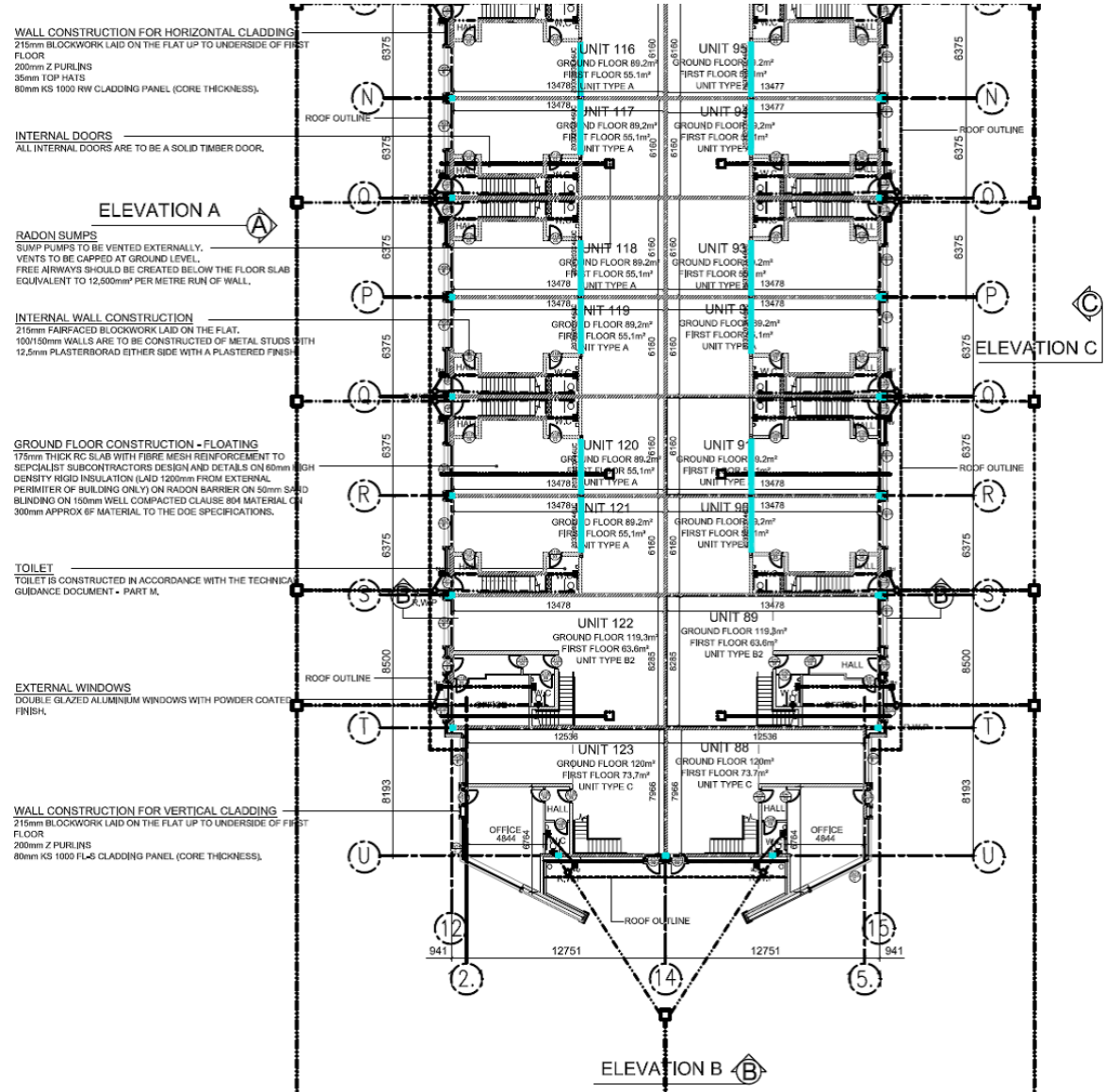
Ground Floor Plan 2- Cut Through Grid Line M-M
