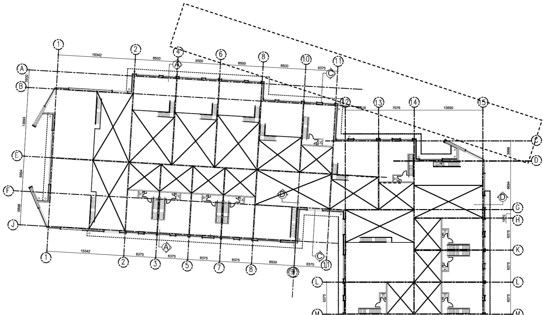
First Floor Plan 1 - Cut Through Grid Line M-M
