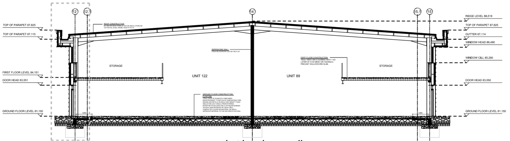
Section B-B Dashed line shows Wall Section 2
