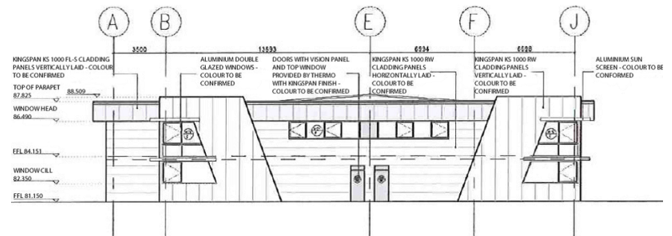
Elevation F-F
