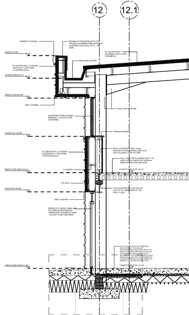
Wall Section 2 - Dashed line shows Detail 2
