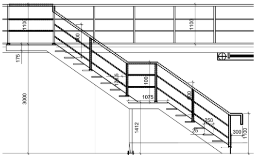
Steel Stair Type 1 - Section A-A
