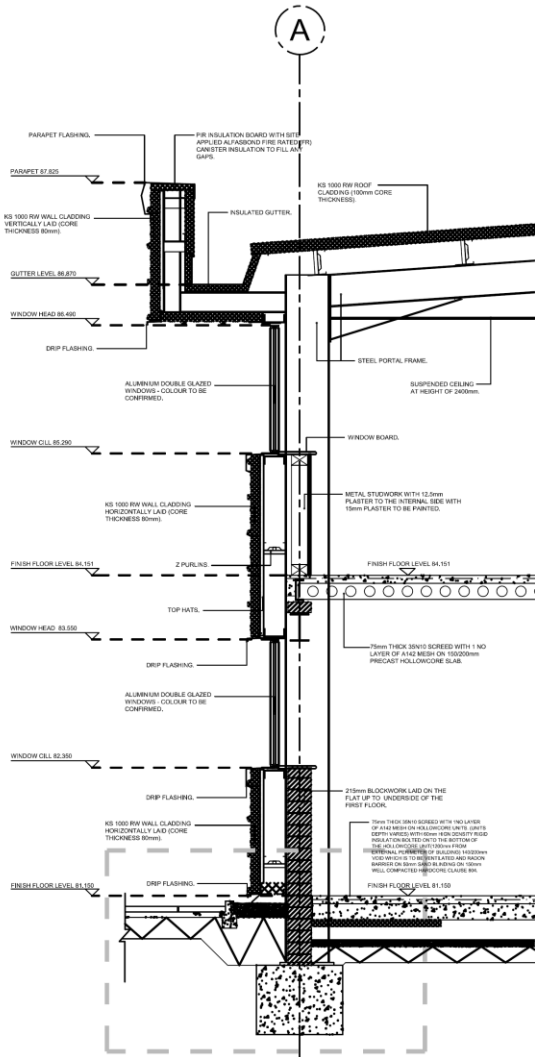
Wall Section 1 - Dashed line shows Detail 1
