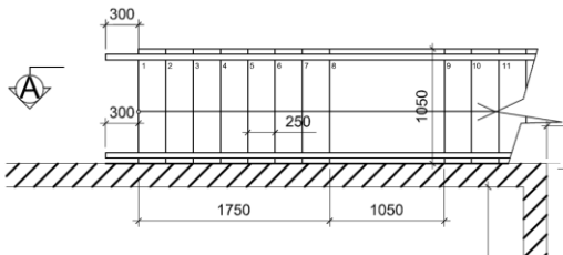
Steel Stair Type 1 - Plan - Ground Floor
