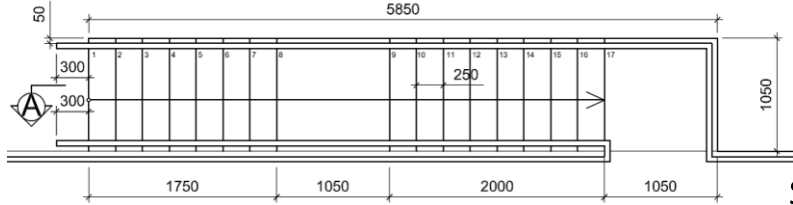
Steel Stair Type 1 - Plan - Ground Floor
